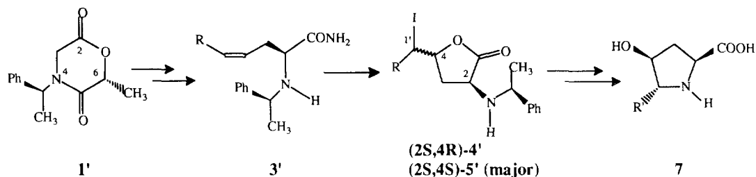
Scheme 2. Where a) : R and R' = H ; b) : R = CH 2 OBn and R' = CH 2 OH.
