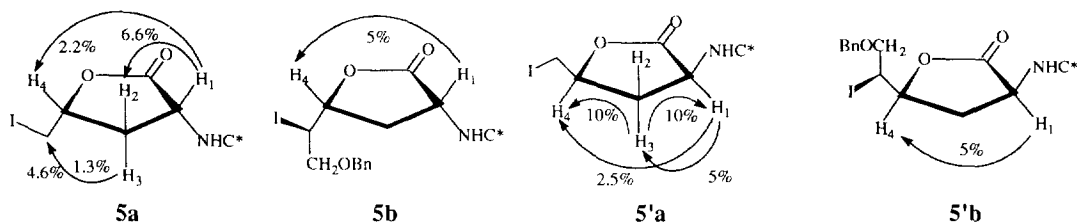
Figure 1. Where C* represents the ( S )-phenylethyl chiral group.
